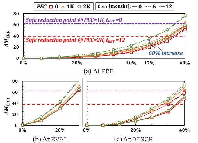
Figure 8: Effect of reducing each read-timing parameter.
