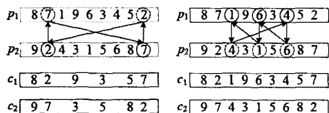
(c) 2nd step of cycle crossover (d) 3rd step of cycle crossover
