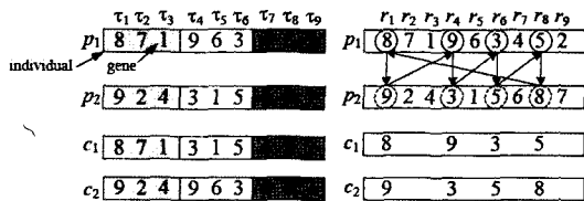
(a) two-point crossover (b) 1st step of cycle crossover
